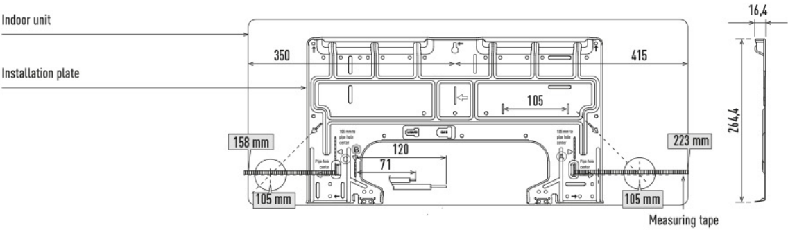
Relative position between the indoor unit and the installation plate
